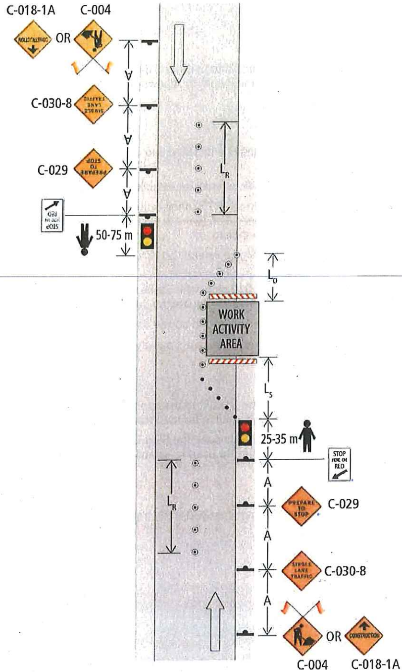
Figure 7.9: Lane Closure with AFADs – Short and Long Duration
